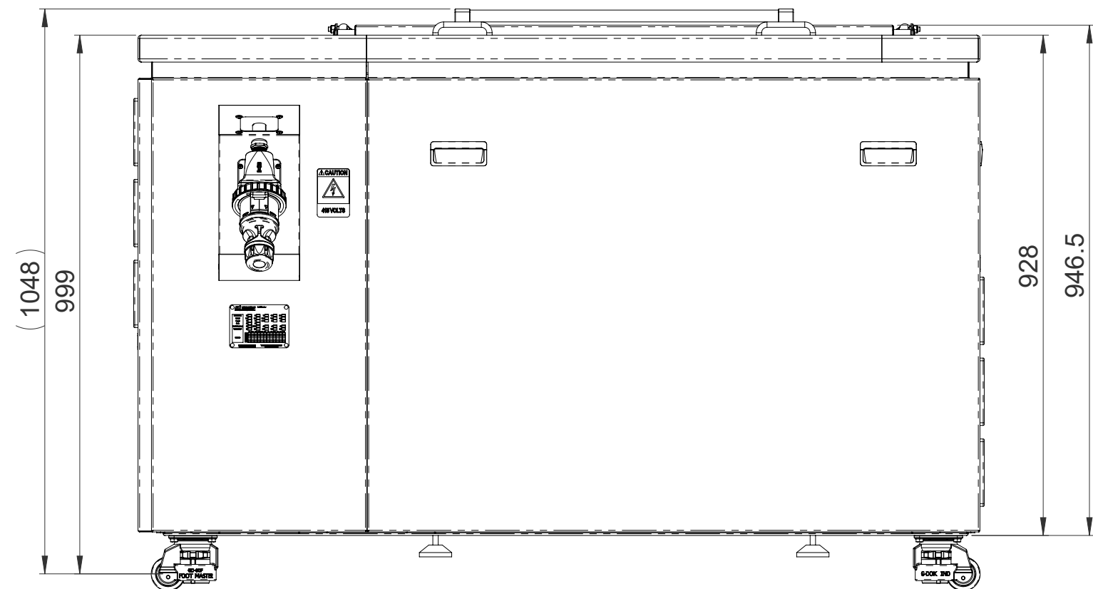
BACK VIEW
