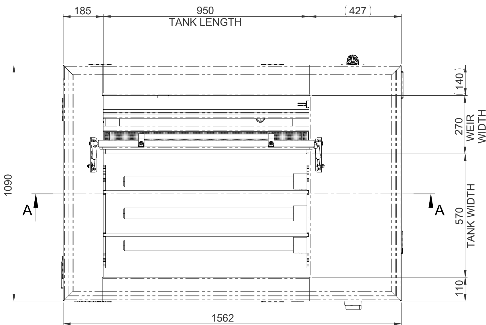
TOP VIEW
