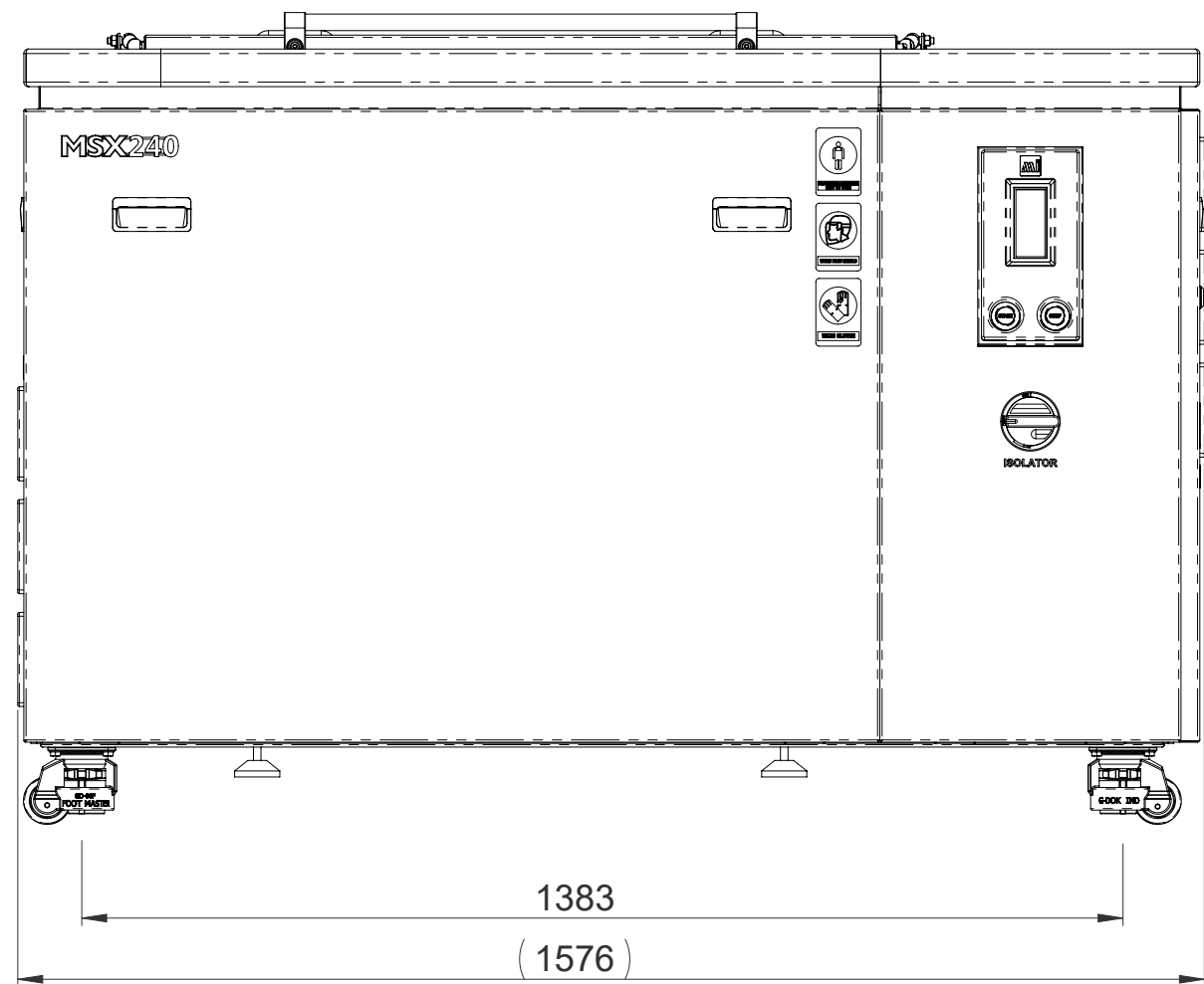
FRONT VIEW
