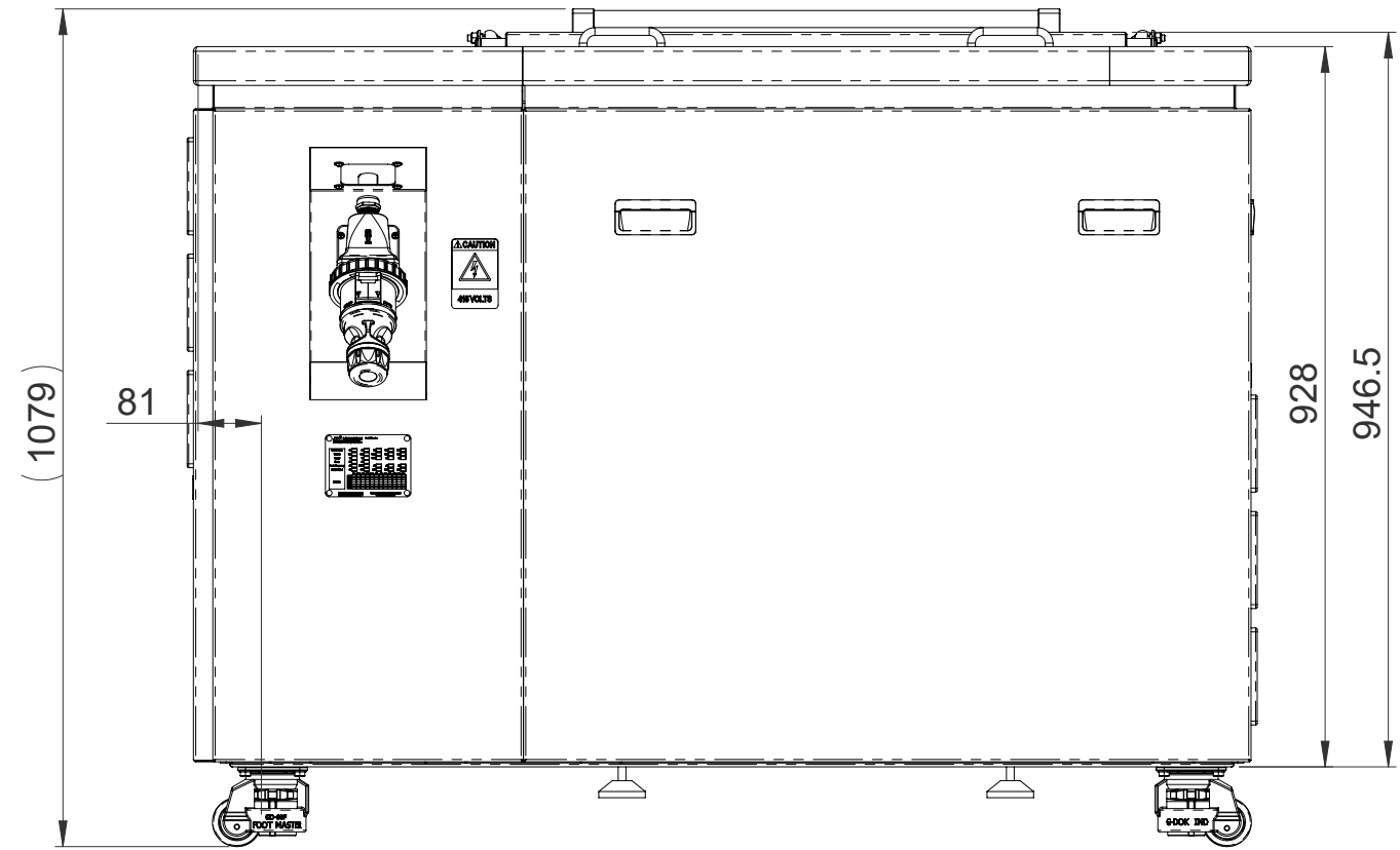
BACK VIEW
