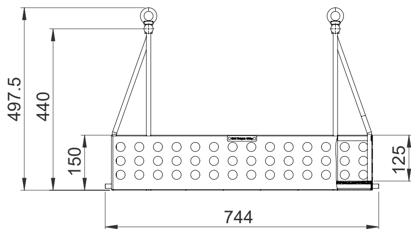
BASKET FRONT VIEW
