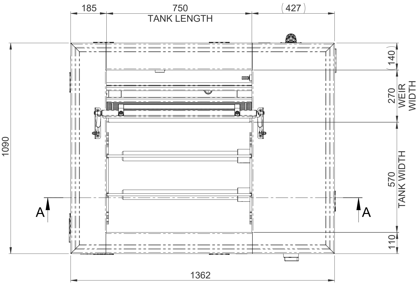
TOP VIEW
