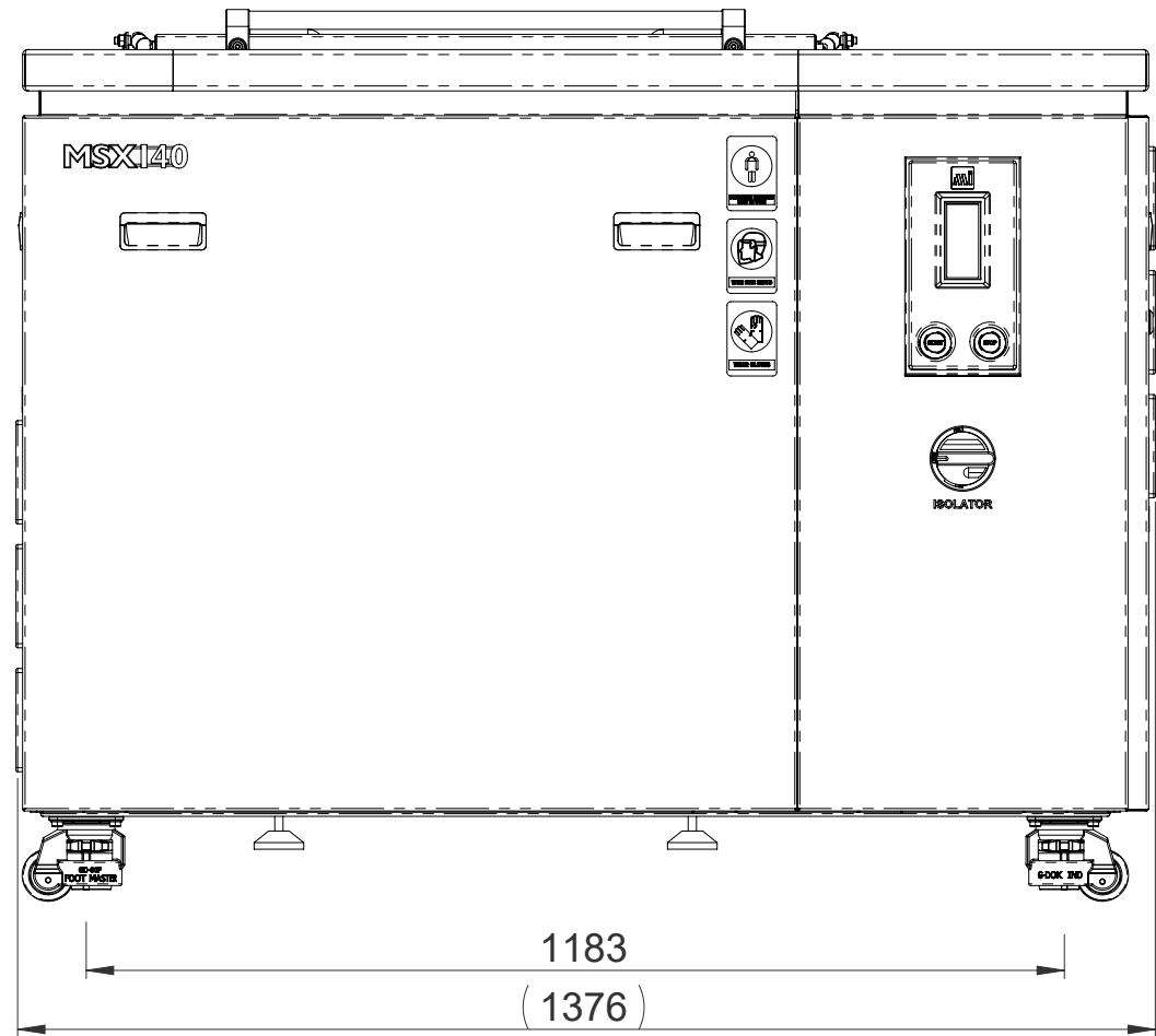
FRONT VIEW
