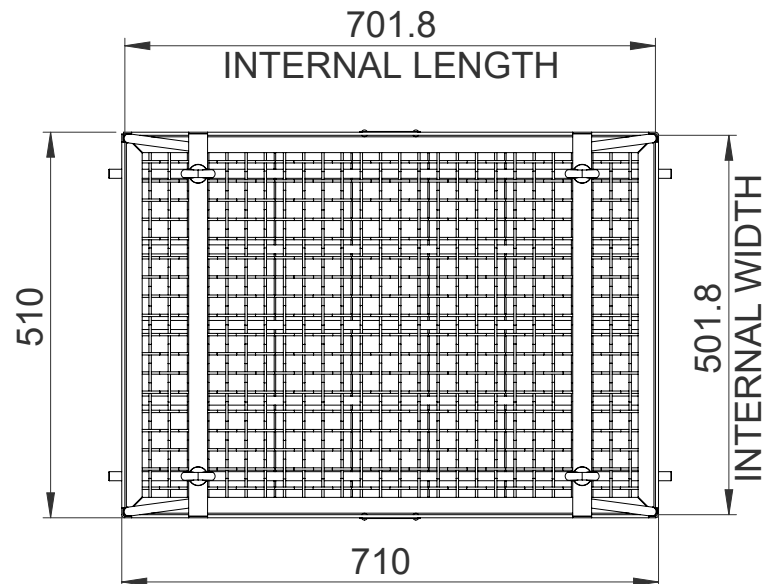
BASKET TOP VIEW
